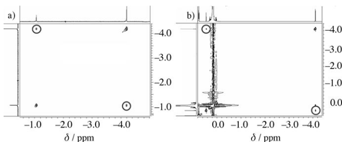
Figure 2. 2D EXSY NMR spectra of encapsulated cyclopropane; mixing times 300 ms. Spectra were obtained from solutions of a) 1·1 (2 mM) or b) 1·2 4 ·1 (2 mM) in (gas-saturated) [D 12 ]mesitylene. The signal at \delta = +0.45 ppm in (b) corresponds to the guest near the belt of glycoluril molecules while the large signal at \delta \approx 0.2 ppm is that of free cyclopropane in [D 12 ]mesitylene. Cross-peaks are circled.
